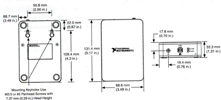
Figure 1. NI cDAQ-9171 Dimensions
